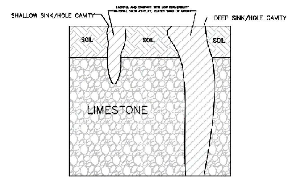
SHALLOW & DEEP SINK HOLE/CAVITY REPAIR & MAINTENANCE DETAIL CONTACT GEOTECHNICAL ENGINEER FOR FURTHER EVALUATION & ADDITIONAL REMEDIATION MEASURES IF NEEDED
